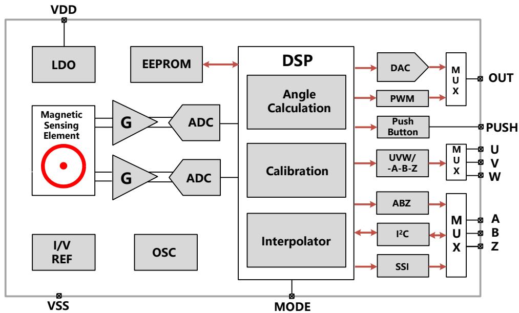
Figure-3: Block Diagram
